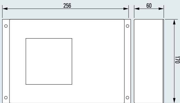
Weatherproof Indicator
